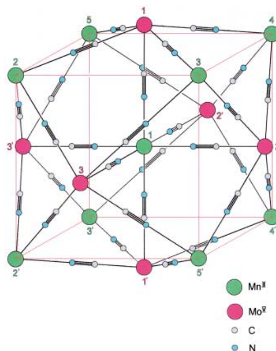
Figure 1. The structure of the Mo_6Mn_9(\mu-CN)_{30} core of the cluster 1 (symmetry group C_2 ) which contains three nonequivalent molybdenum sites. A similar core is found in 2 (symmetry group S_6 ), which contains six equivalent tungsten sites, and in 3 .
