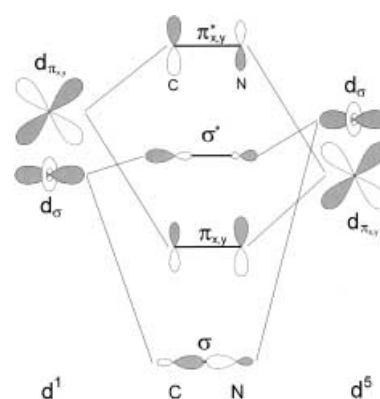
Figure 4. Definition of the d_0 , d_{\pi_x} , and d_{\pi_y} orbitals on the 4d(M) and 3d(M') sites for a given metal pair M-(CN)-M' ( \pi_y -type orbitals lie in the plane perpendicular to the drawing). The two basic electron-transfer pathways ( \sigma and \pi ) through the cyanide bridge are outlined by the thin oblique lines. The corresponding transfer parameters describe the electron transfer in the chains: \beta_\sigma = d_0(M)-\sigma^*, \sigma(CN)-d_0(M') , \beta_\pi \equiv \beta_{\pi_x} = \beta_{\pi_y} = d_{\pi_x}(M)-\pi^*, \pi(CN)-d_{\pi_x}(M') .
